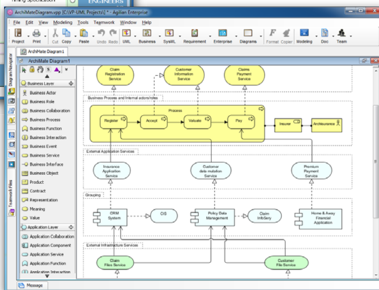
ArchiMate
